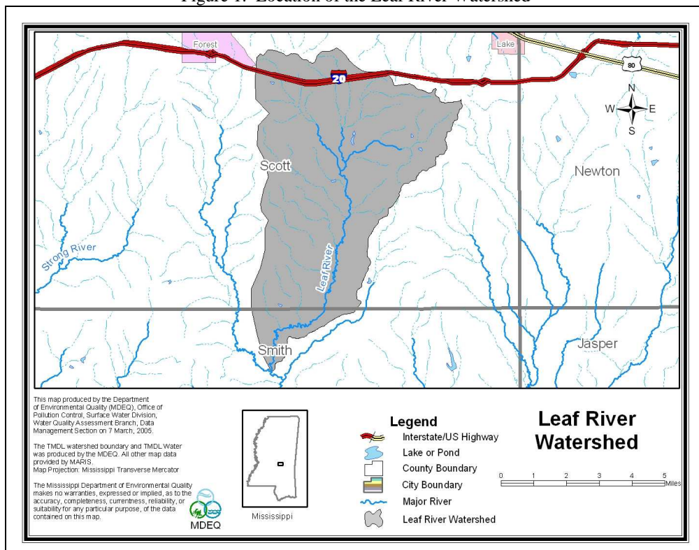
Figure 1. Location of the Leaf River Watershed
