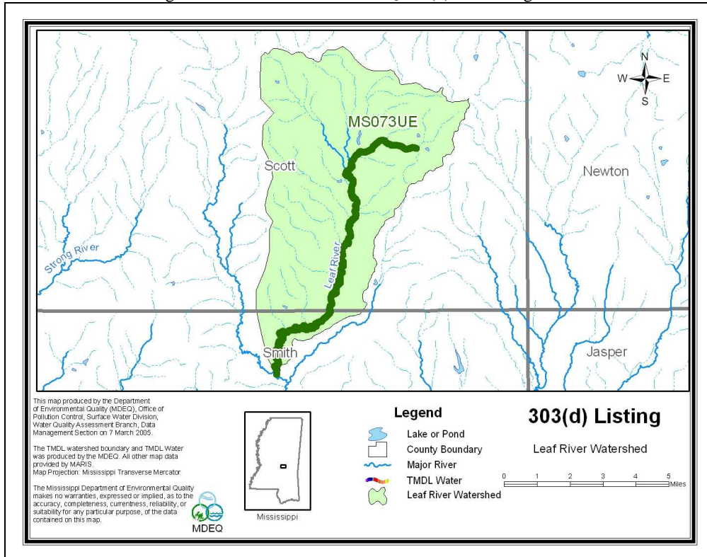
Figure 2. Leaf River Watershed §303(d) Listed Segment
