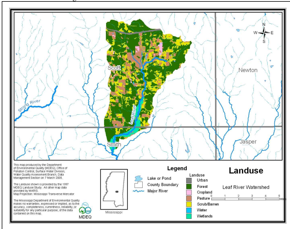
Figure 3. Leaf River Watershed Landuse Distribution
