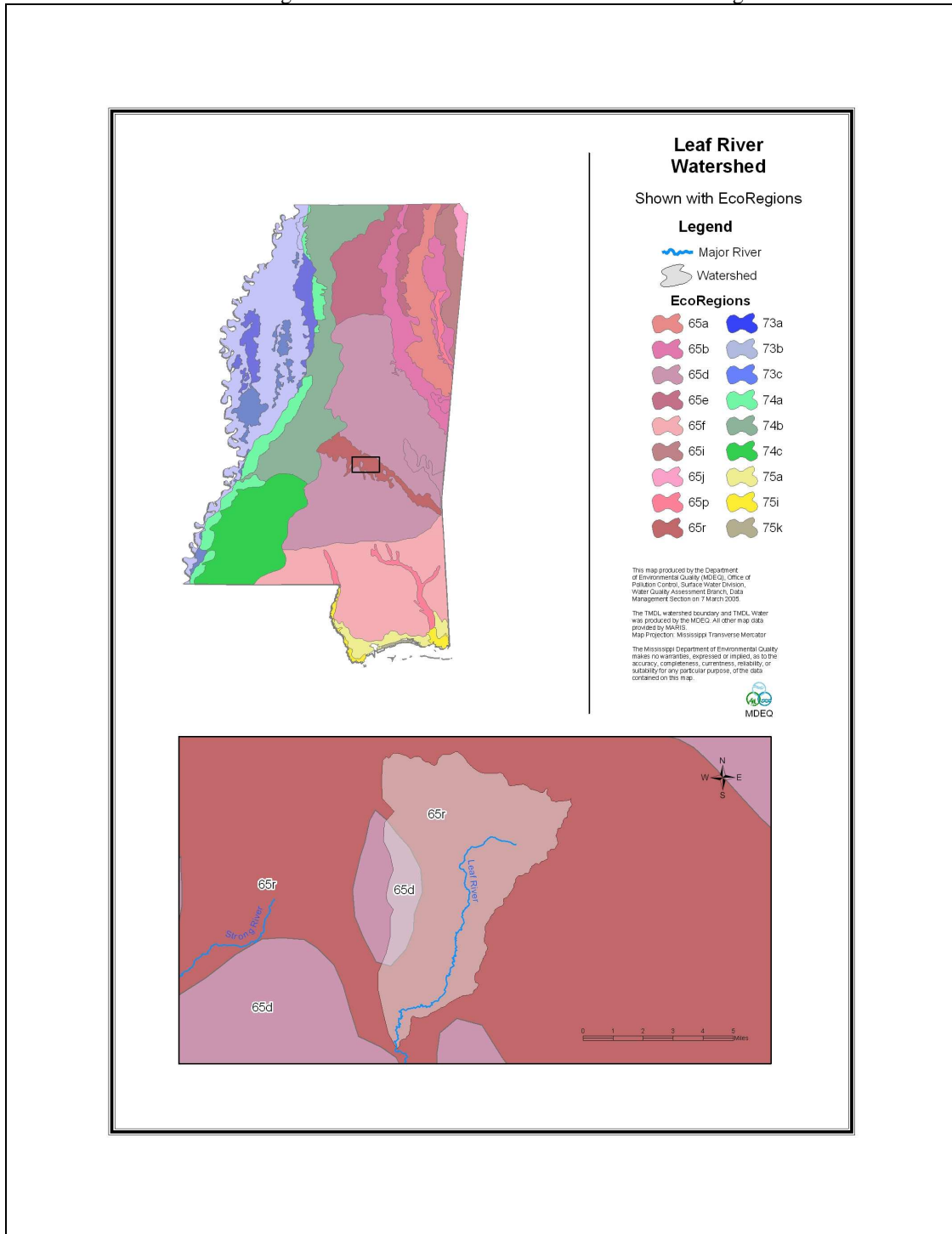
Figure 5. Leaf River Watershed with Level IV Ecoregions
