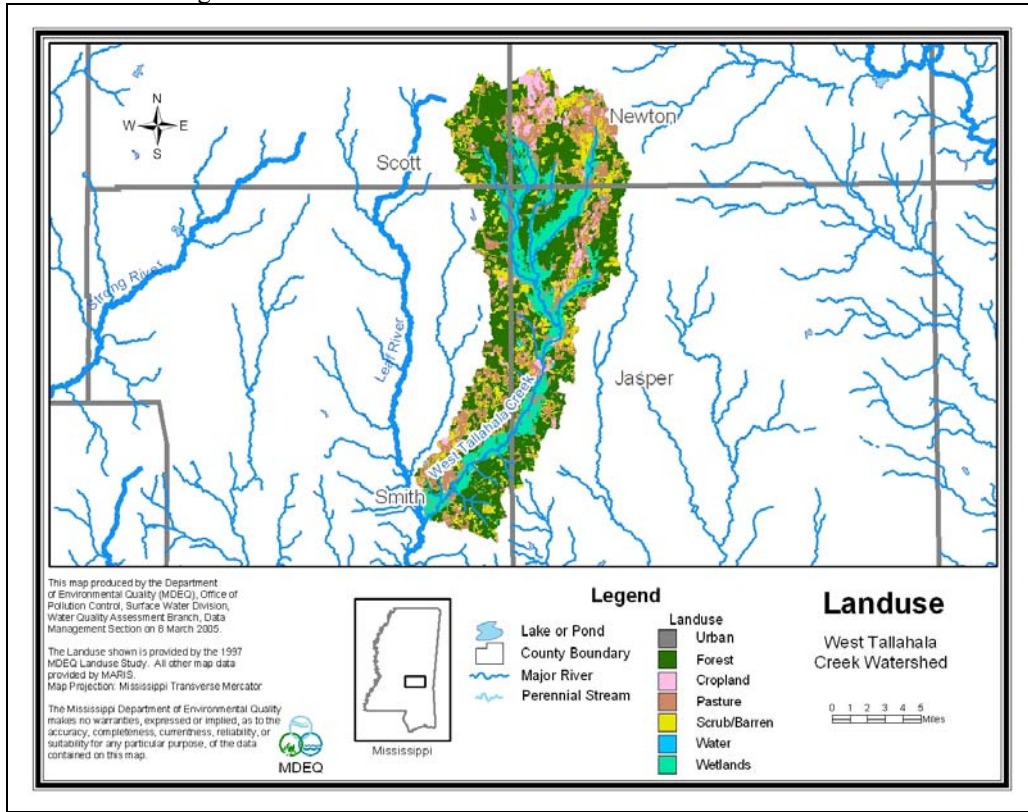
Figure 3. West Tallahala Creek Watershed Landuse Distribution
