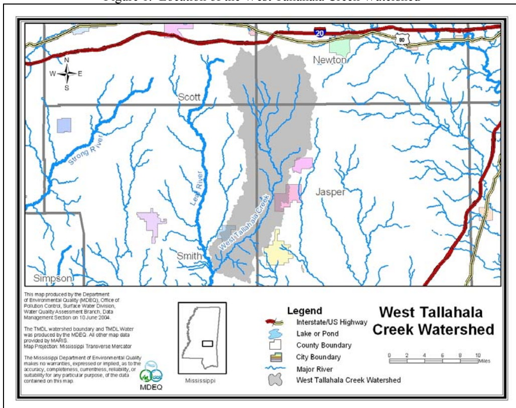
Figure 1. Location of the West Tallahala Creek Watershed
