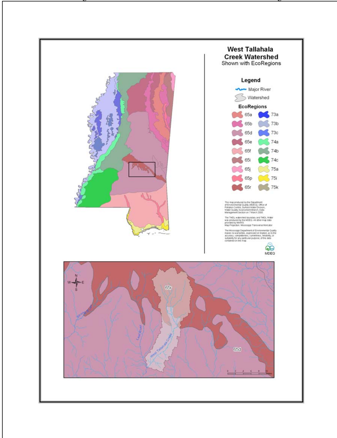
Figure 5. West Tallahala Creek Watershed with Level IV EcoRegions
