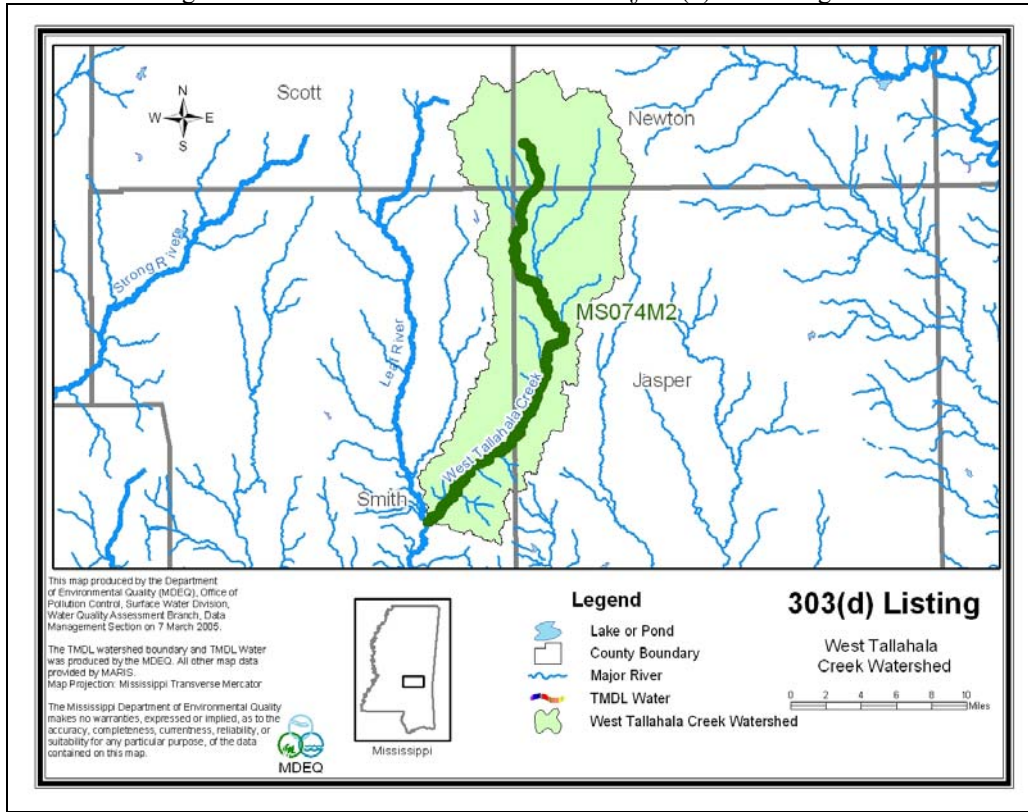
Figure 2. West Tallahala Creek Watershed §303(d) Listed Segment
