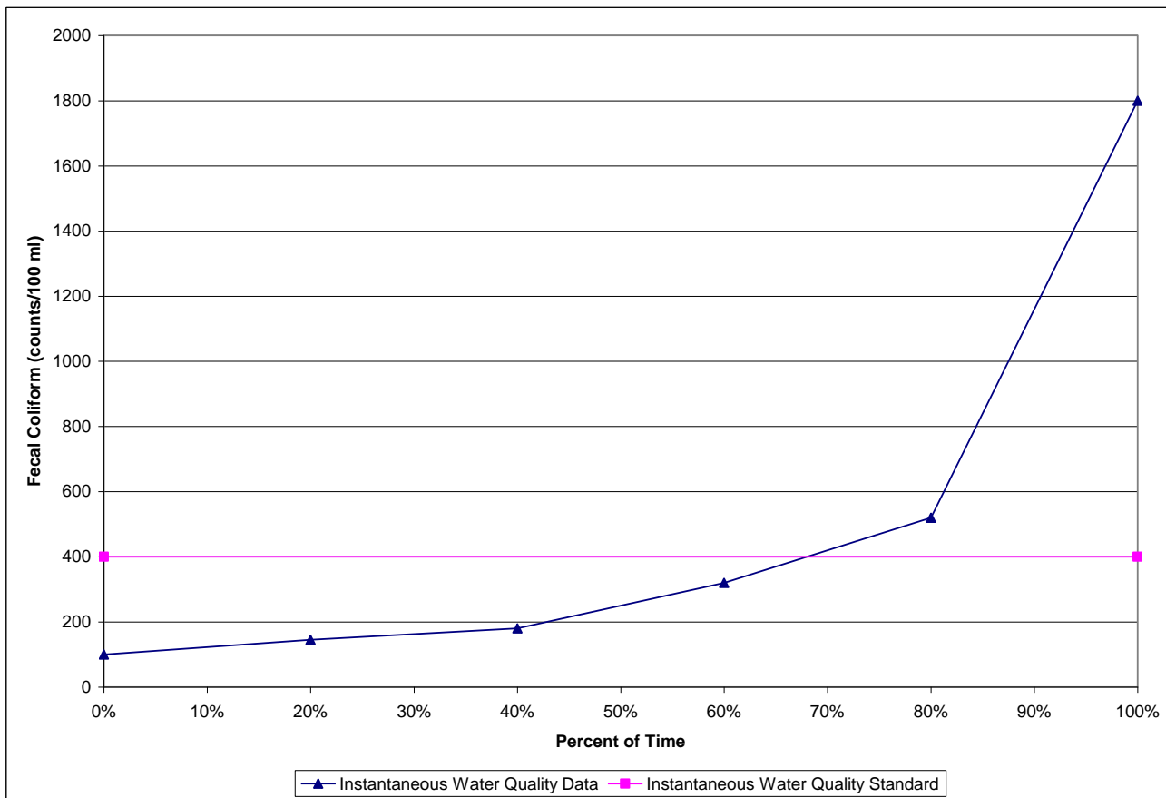
Figure 6. 10% Test Curve for Station PR-10, Summer 2001
