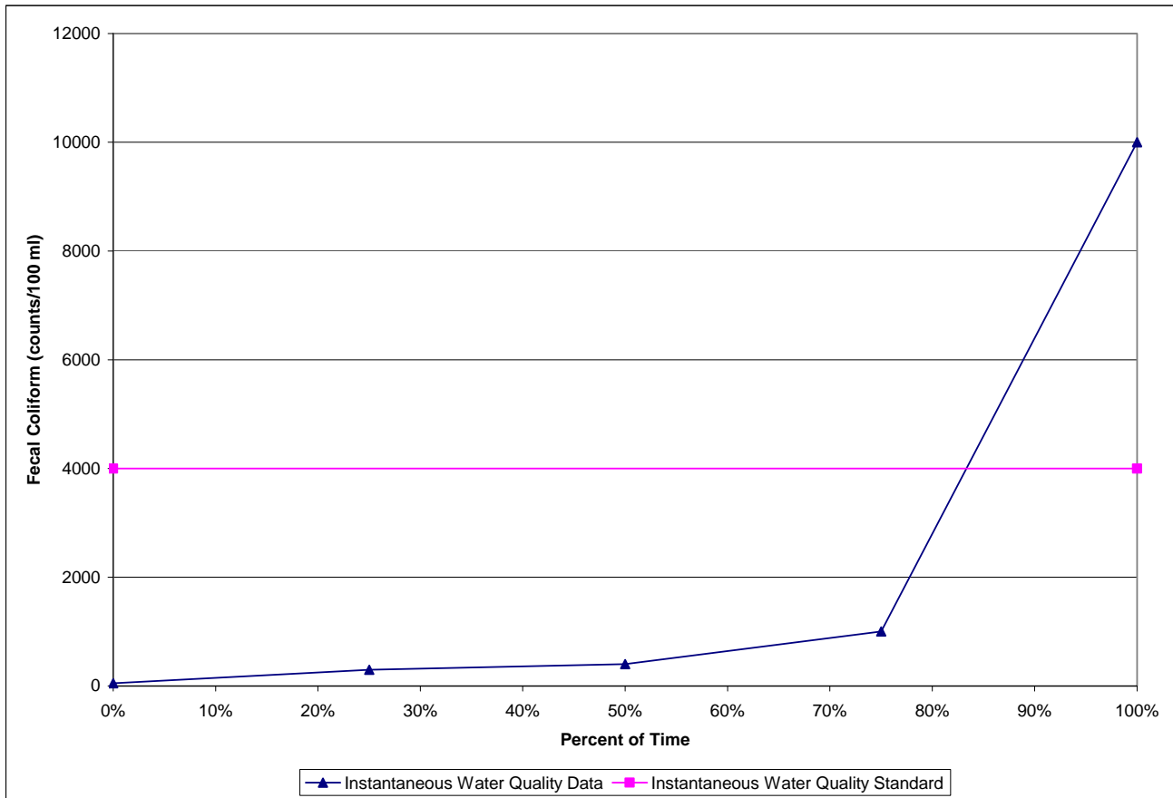
Figure 5. 10% Test Curve for Station PR-8, Winter 2000
