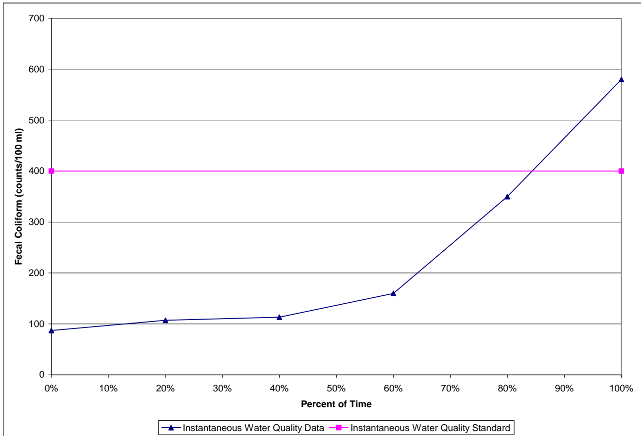
Figure 6. 10% Test Curve for Station PR-8, Summer 2003
