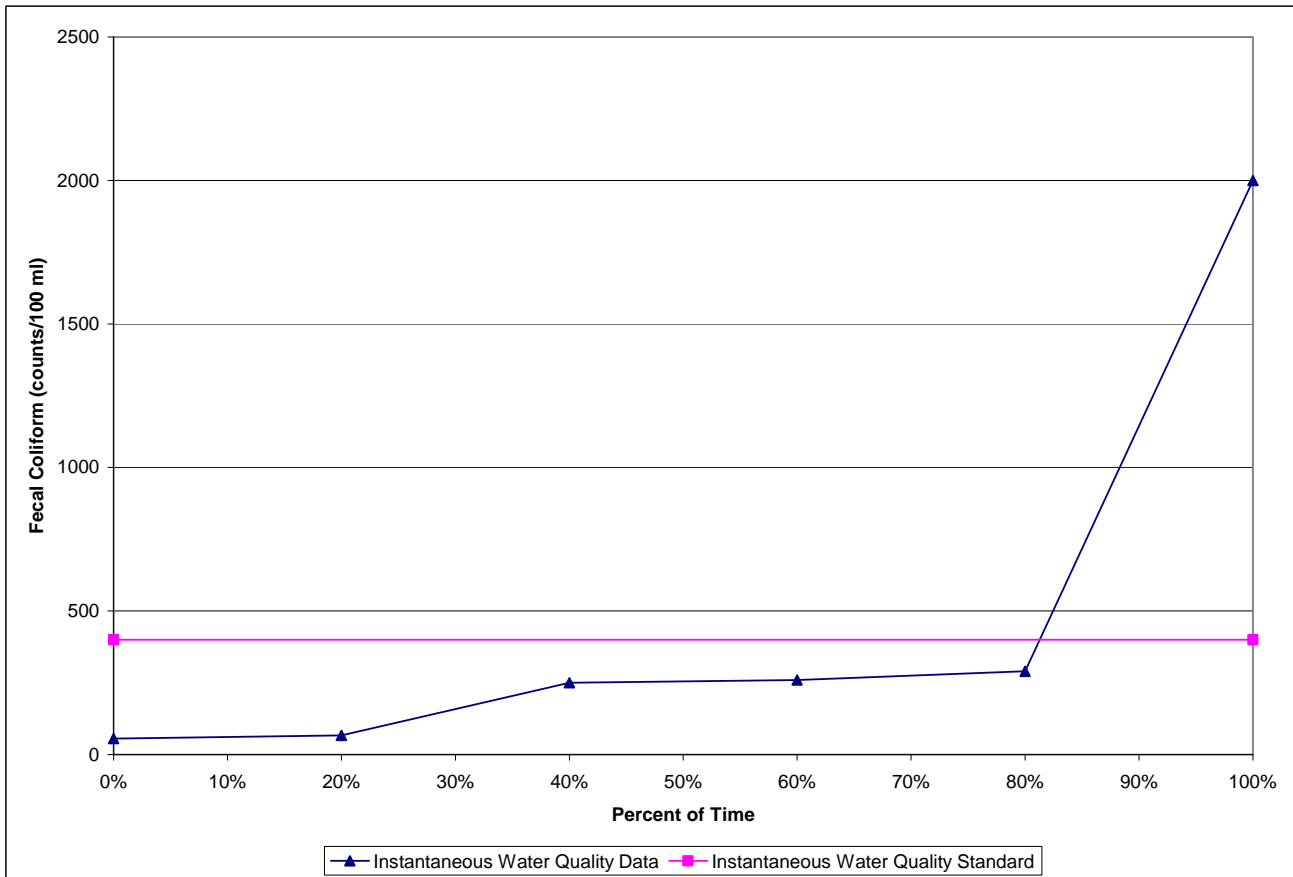
Figure 5. 10% Test Curve for Station PR-48, Summer 2003
