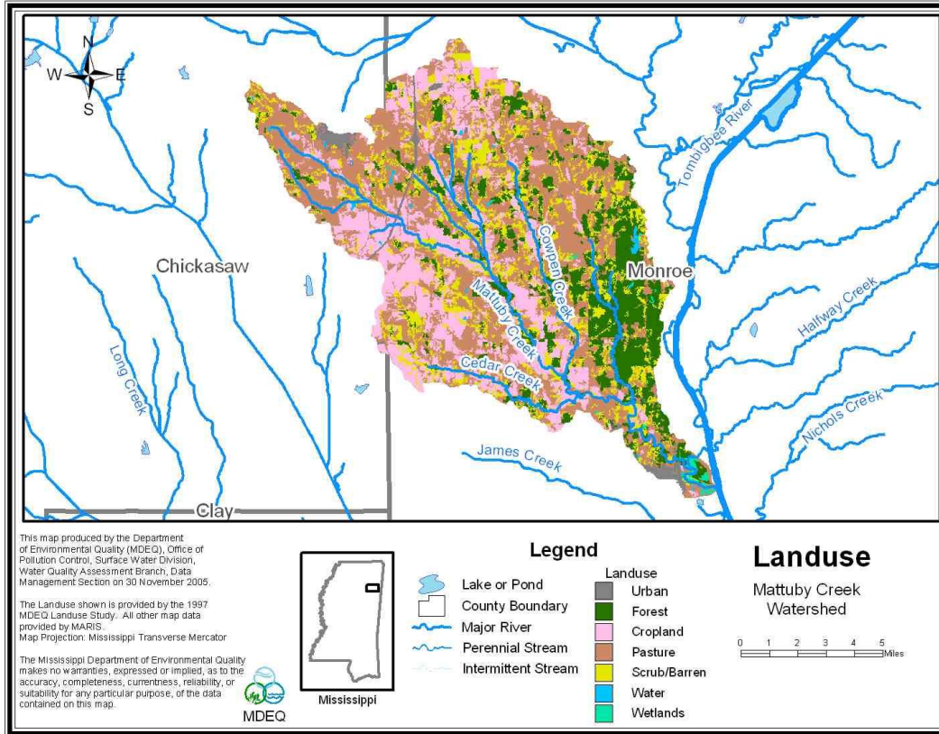
Figure 6. Land Use Distribution Map for Mattubby Creek Watershed
