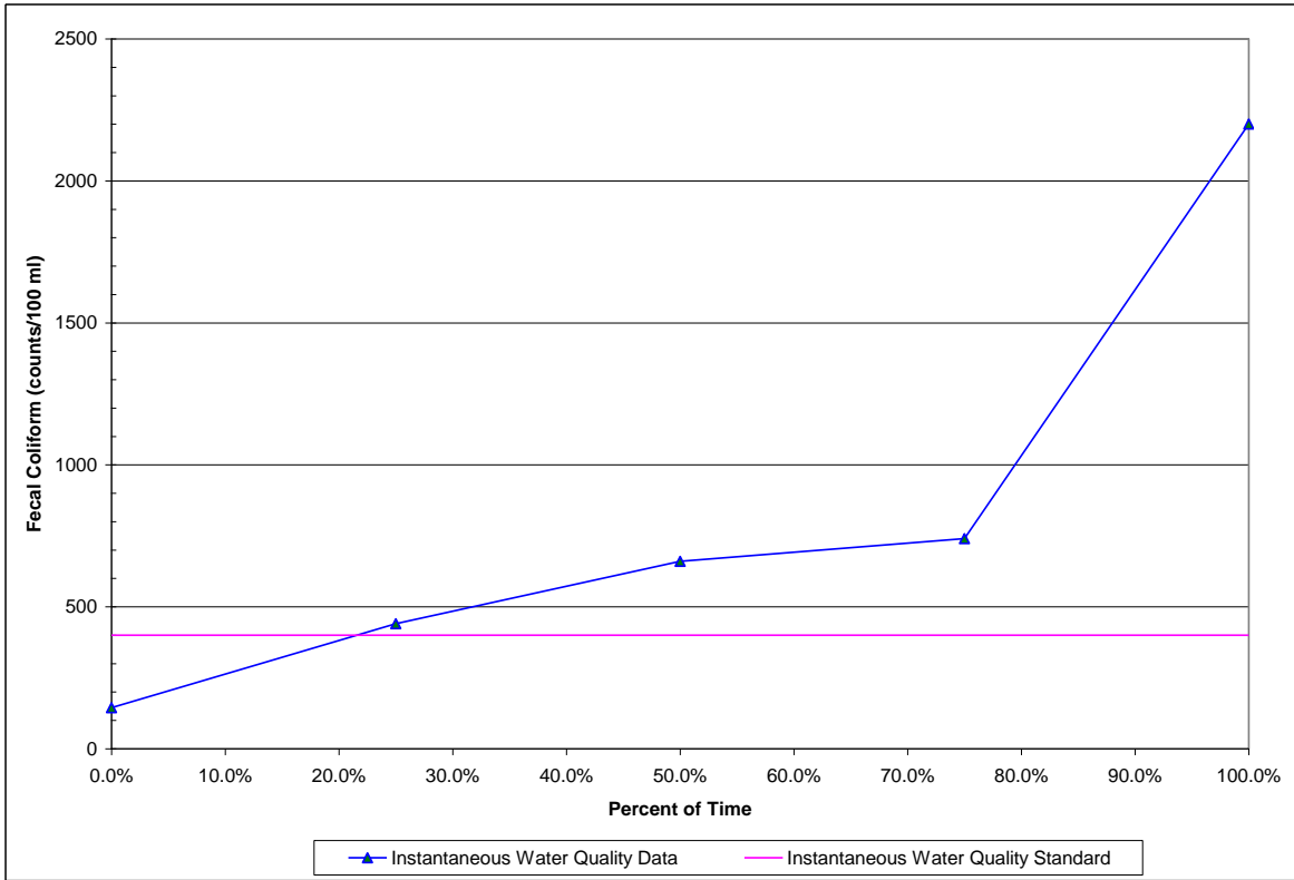
Figure 5. 10% Test Curve for Station 52, Summer 2003
