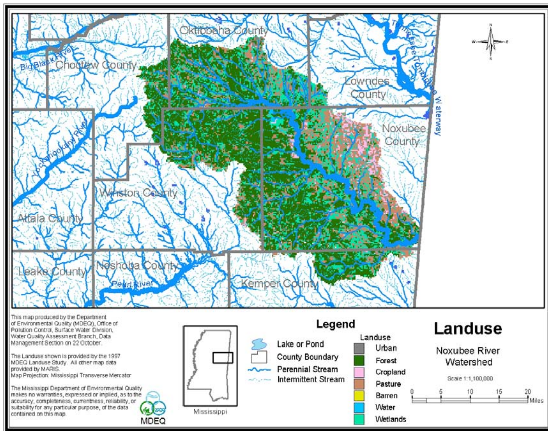
Figure 5. Landuse Distribution Map for the Noxubee River Watershed
