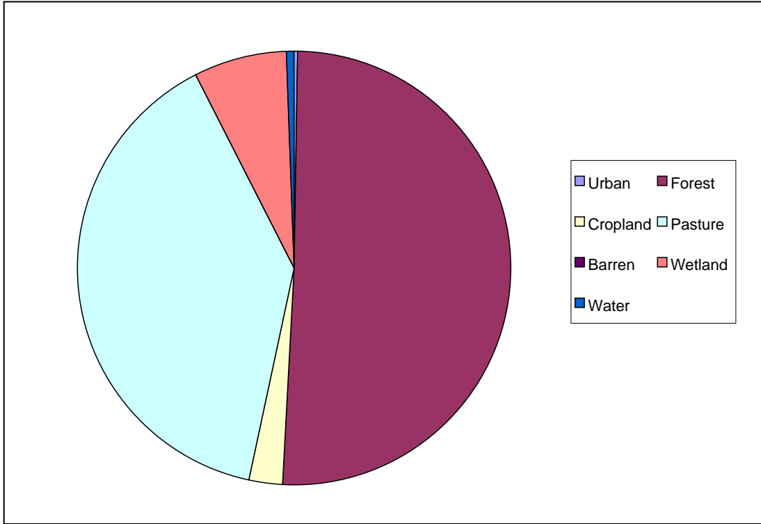
Figure 2. Noxubee River Watershed Landuse
