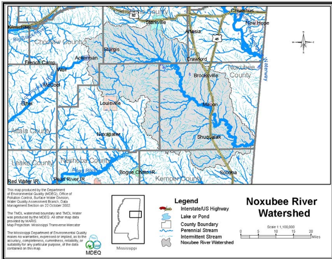
Figure 1. Location of Noxubee River Watershed
