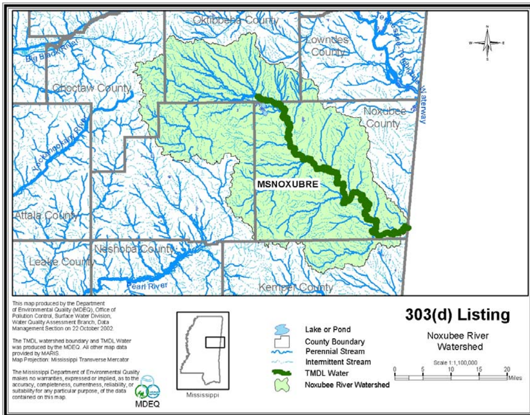
Figure 3. Noxubee River 303(d) Listed Segment
