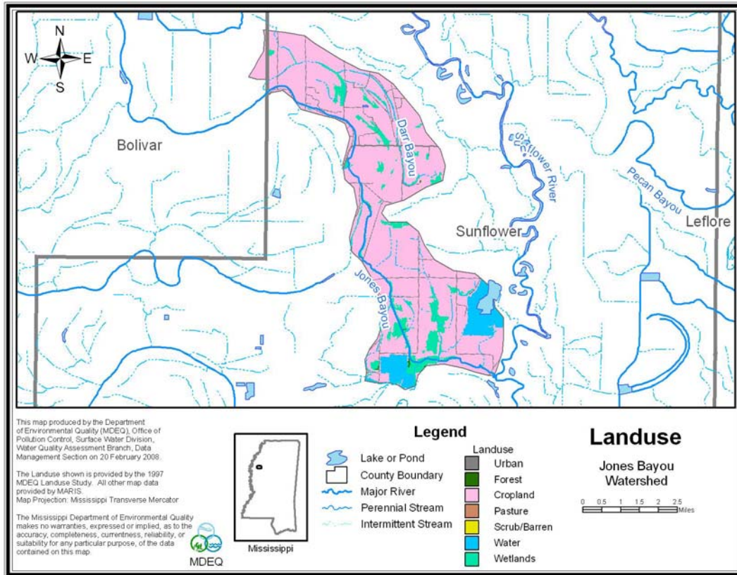
Figure 3. Jones Bayou Watershed Landuse
