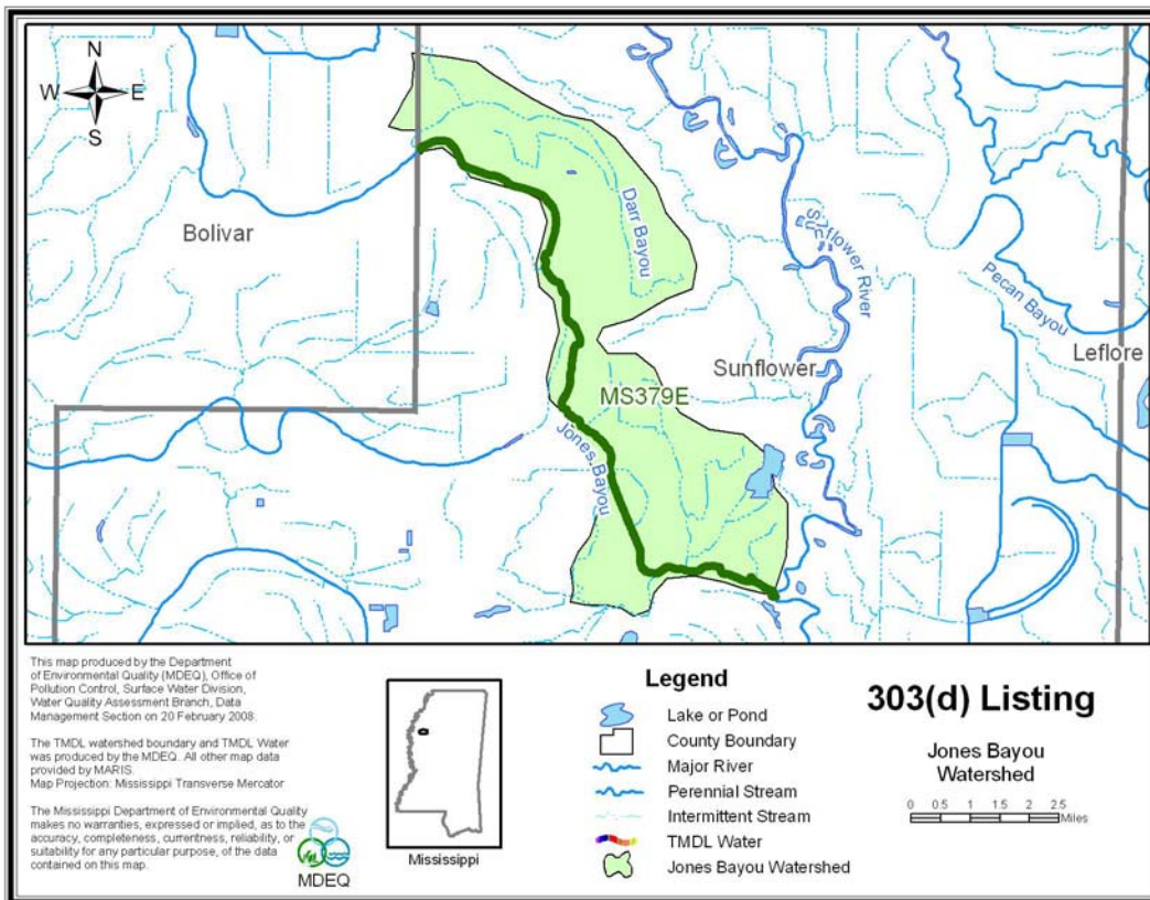
Figure 2. Jones Bayou §303(d) Listed Segment
