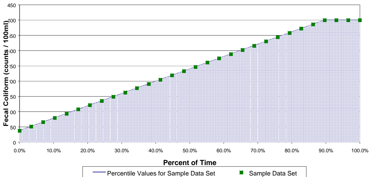
Figure 4. Theoretical Capacity Curve
