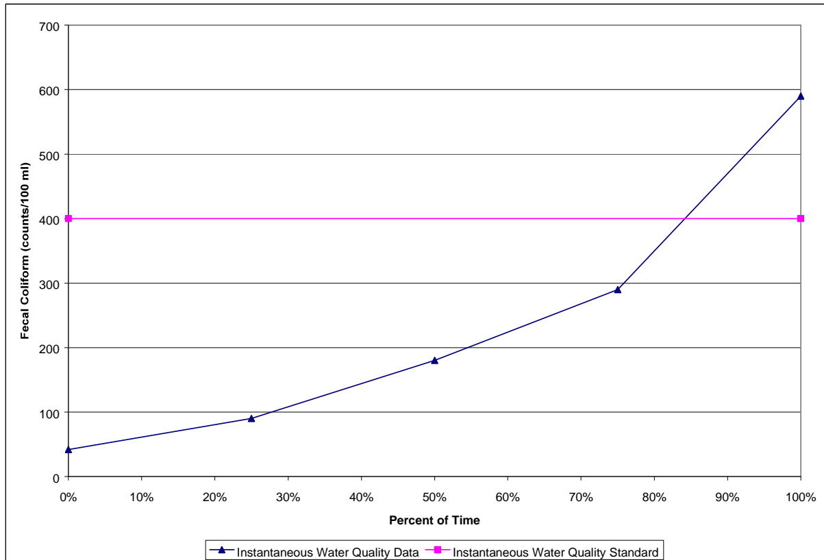
Figure 5. 10% Test Curve for Station FTN-45, Summer 2003
