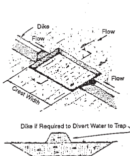
Section A-A Excavated Earth Outlet Sediment Trap
