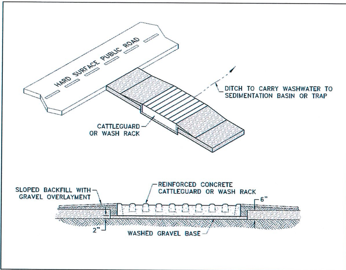
Figure CEP-2 Construction Exit with Wash Rack
