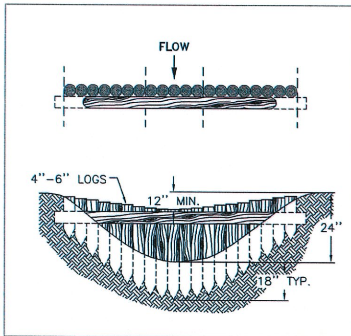
Figure CD-3 Typical Log Check Dam
