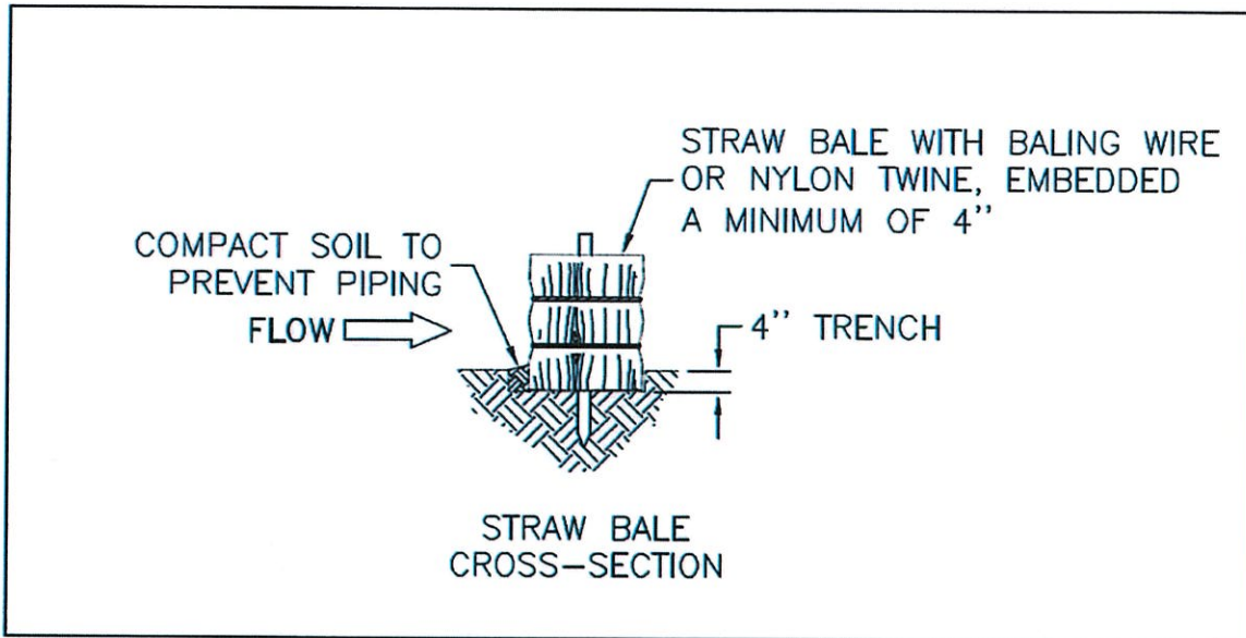
Figure CD-4 Typical Hay Bale Check Dam
